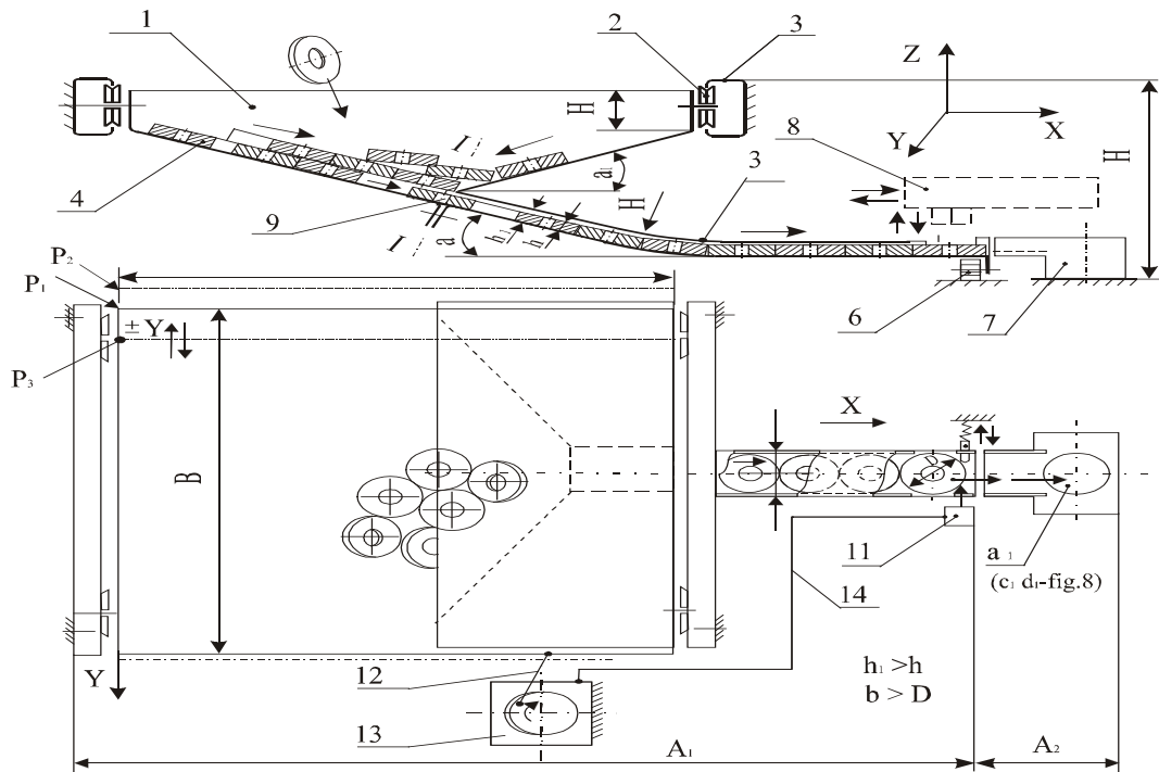
Figure 12: 1. Parts stack bin; 2. Roller; 3. Guide roller; 4. Component parts (of the 2, 3 and 4 type in Figure 11); 5. Trough; 6. Roller; 7. Assembly fixture (working positions a_1 , c_1 and d_1 ); 8. Robot arm (manipulator); 9. Gap; 10. Lock; 11. Electrical sensor; 12. Connecting rod – crank mechanism; 13. Motor; 14. Electrical wiring.
